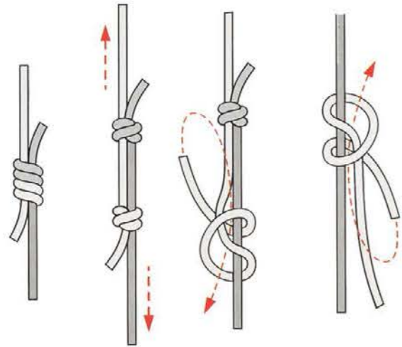
DOUBLE FISHERMAN'S KNOT
