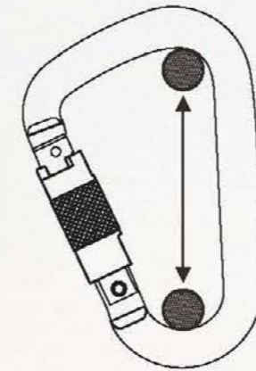
2. MAJOR AXIS STRENGTH WITH GATE CLOSED AND LOCKED
