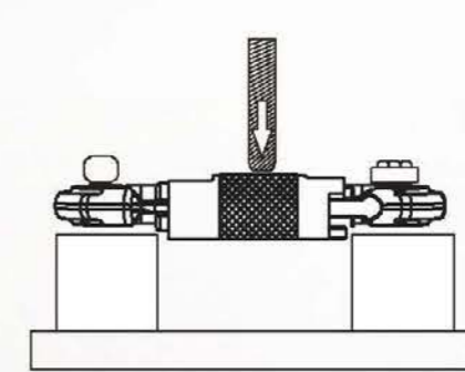
5. GATE SIDE-LOAD RESISTANCE TEST
