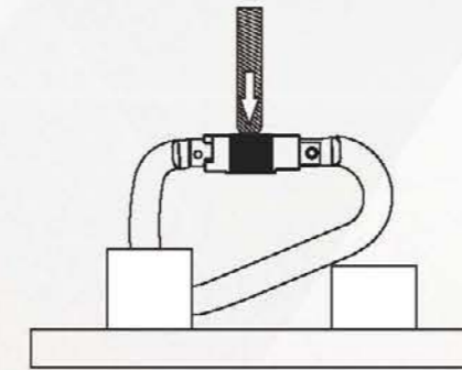
4. GATE FACE RESISTANCE TEST
